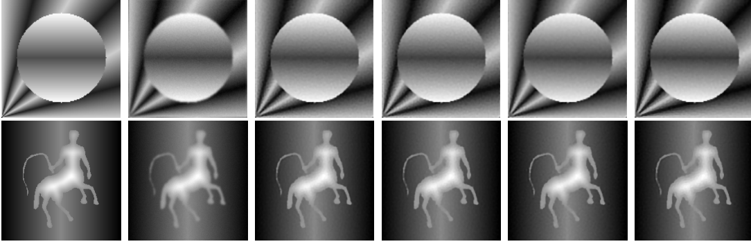
Figure 1: From left to right, the original image, the blurry and noisy, and the deblurring images using the total variation (TV) model [27], the analysis based model (1.5), the general model (1.13) with q = 1 and q = 2 . The PSNR values of the recovered images for the first example (row one) are 34.32 (TV), 34.46 (Analysis), 35.12 ((1.13) with q = 1 ) and 34.87 ((1.13) with q = 2 ). The PSNR values for the second example (row two) are 36.28 (TV), 36.52 (Analysis), 36.74 ((1.13) with q = 1 ) and 36.77 ((1.13) with q = 2 )
