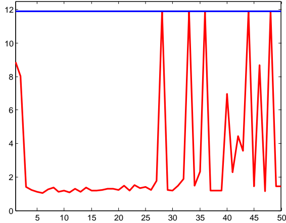
Figure 1: Horizontal axis represents the iteration number k , while the vertical axis represents \tau_k . The red line represents \tau_k of EPIHT-LS algorithm; the blue line represents global Lipschitz constant L .
