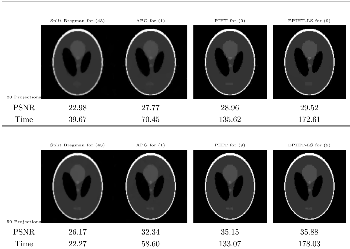
Figure 2: CT image reconstruction results. The first row shows the reconstruction results using 20 projections, and the second row shows the reconstruction results using 50 projections. The running time is listed in seconds .
