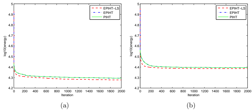
Figure 3: Energy evolving curves of CT image reconstruction, (a) for 20 projections, (b) for 50 projections.
